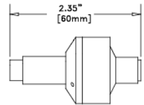
1/2" OD Smooth tube (HPM-2002-07)
